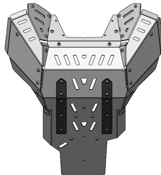
ALUMINUM TRAIL ENGINE GUARD Ref.: 2CP0900090
